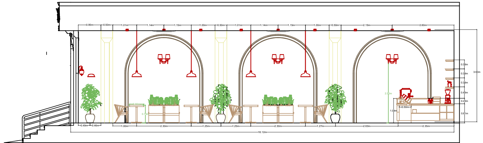
LEFT SIDE ELEVATION ZA CONSTRUCTION (YOUTUBE) UNITS -Meter
