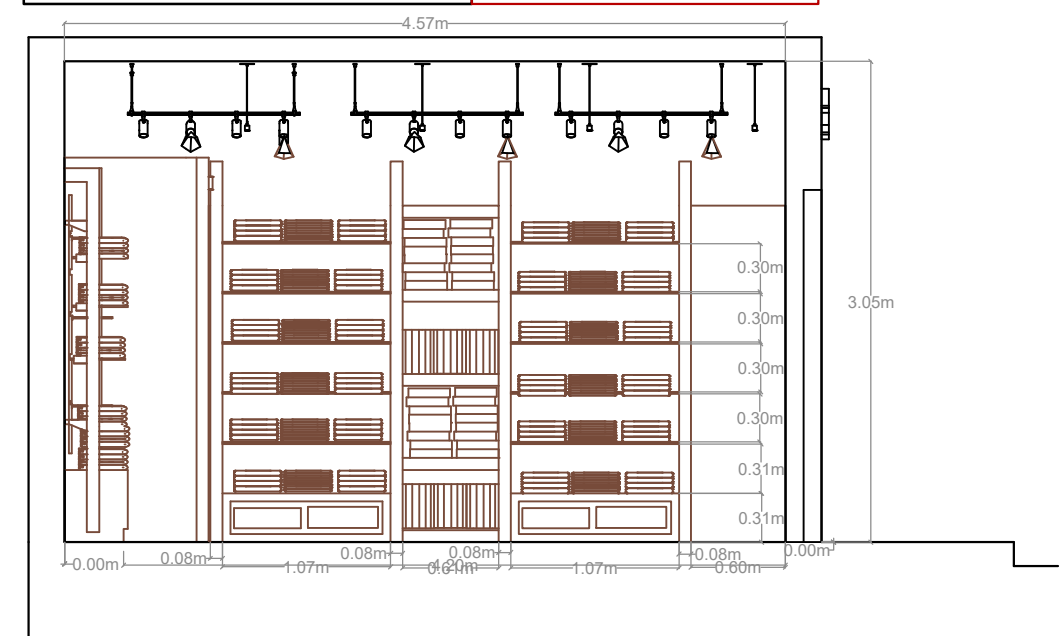
RIGHT SIDE ELEVATION ZA CONSTRUCTION (YOUTUBE) UNITS -Meter
