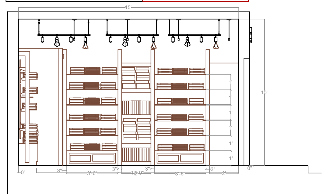
RIGHT SIDE ELEVATION ZA CONSTRUCTION (YOUTUBE) UNITS - FEET
